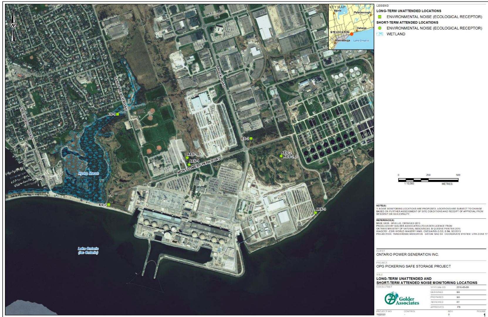
Figure 4.6: Environmental Noise (Ecological Receptors) - Long-term Unattended and Short-term Attended Noise Monitoring Locations
